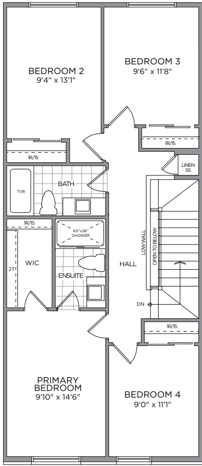
OPT. SECOND FLOOR 4TH BEDROOM
