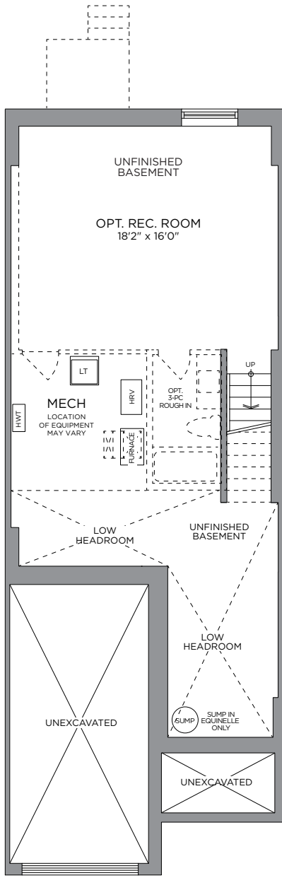
STANDARD BASEMENT OPT. FINISHED REC. ROOM 357 SQ. FT.
