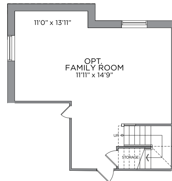
OPT. FINISHED BASEMENT FAMILY ROOM 451 SQ. FT.
