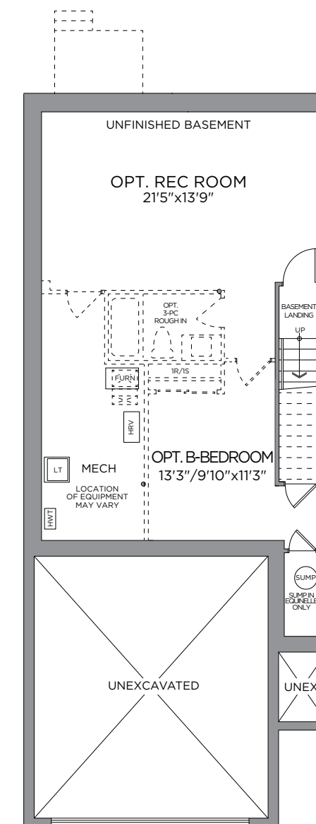
STANDARD BASEMENT OPT. FINISHED BASEMENT 641 SQ. FT.
