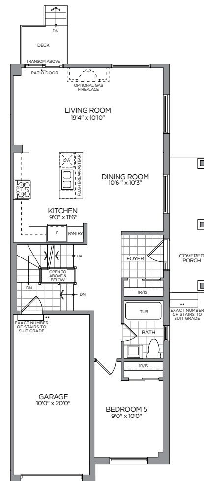
OPT. GROUND FLOOR BED #5 & BATHROOM
