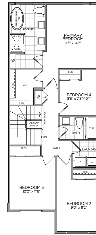
OPT. SECOND FLOOR PRIMARY ENSUITE
