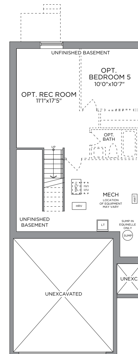
STANDARD BASEMENT PLAN OPT. FINISHED BASEMENT PLAN 468 SQ. FT.
