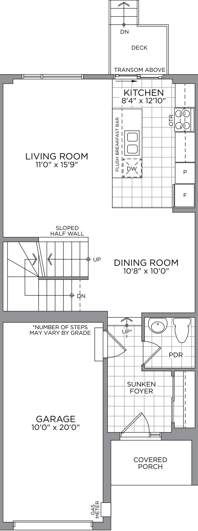
GROUND FLOOR
