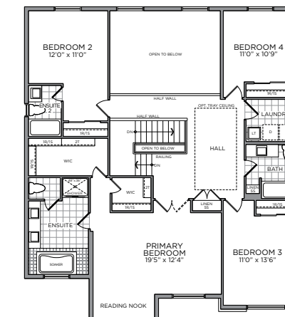
OPT. SECOND FLOOR -215 SQ. FT.
