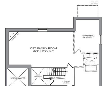
OPT. FINISHED FAMILY ROOM FINISHED AREA 599 SQ. FT.
