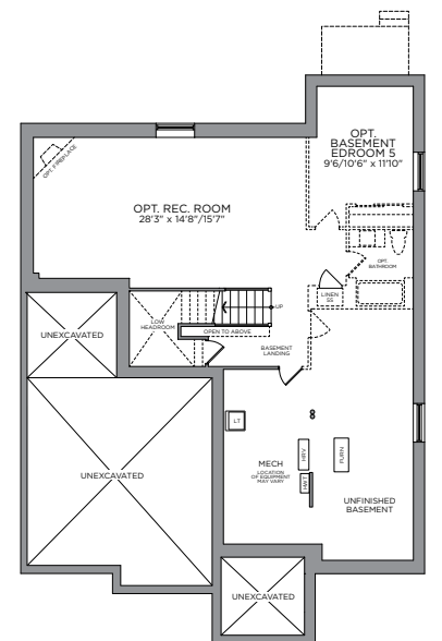
STANDARD BASEMENT PLAN OPT. FINISHED BASEMENT 852 SQ. FT. ELEV. C
