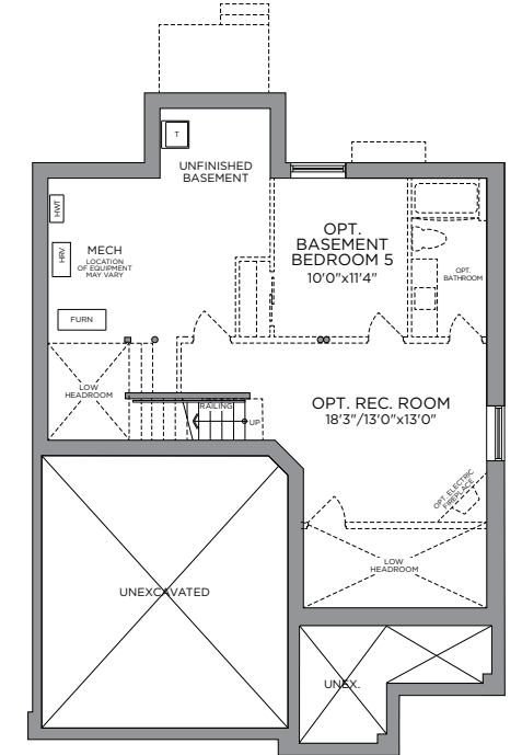
STANDARD BASEMENT PLAN OPT. FINISHED BASEMENT 495 SQ. FT.
