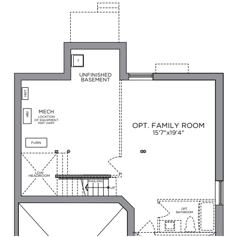
STANDARD BASEMENT PLAN OPT. FINISHED BASEMENT 401 SQ. FT.
