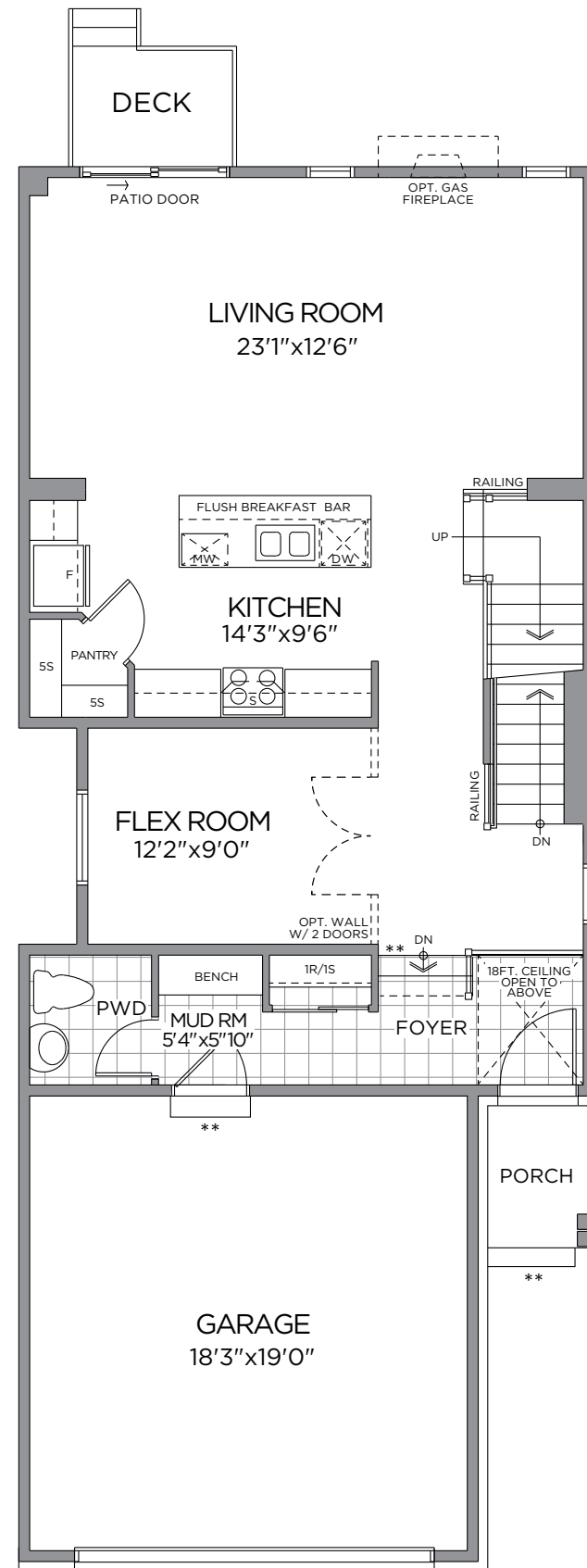
GROUND FLOOR ELEV. C
