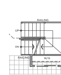
OPT. OPEN STAIRS TO BASEMENT
