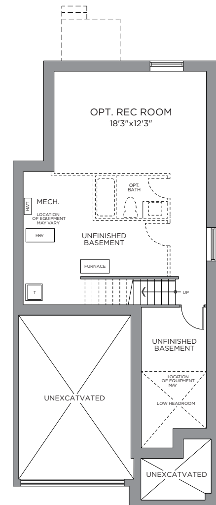
STANDARD BASEMENT PLAN OPT. FINISHED BASEMENT 410 SQ. FT.
