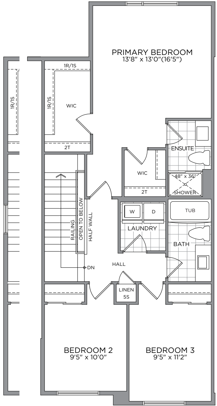
SECOND FLOOR
