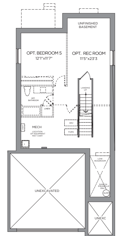
STANDARD BASEMENT ELEV. B OPT. FINISHED BASEMENT FINISHED AREA 624 SQ. FT.
