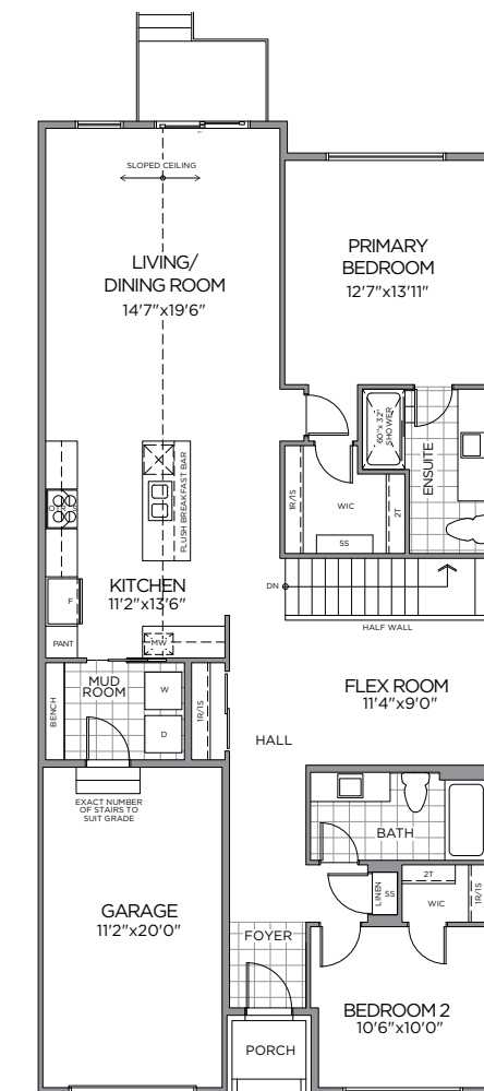
OPT. GROUND FLOOR PLAN ELEV. B
