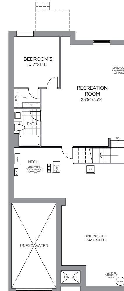
STANDARD BASEMENT ELEV. B OPT. FINISHED BASEMENT FINISHED AREA 750 SQ. FT.
