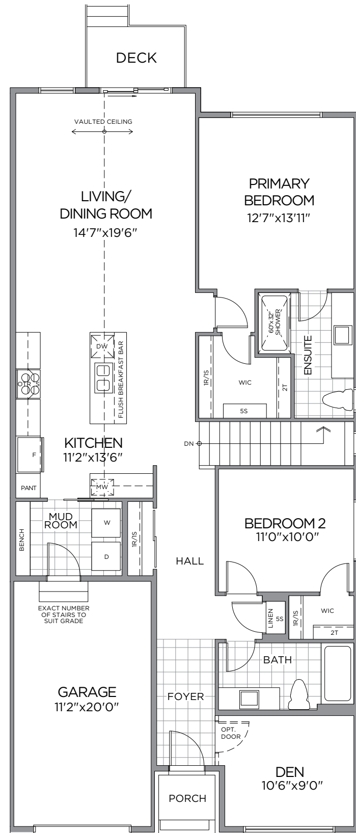
GROUND FLOOR ELEV. B
