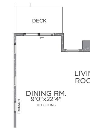
OPT. EXTENDED DINING ROOM 105 SQ. FT.
