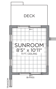
OPT. SUNROOM 105 SQ. FT.
