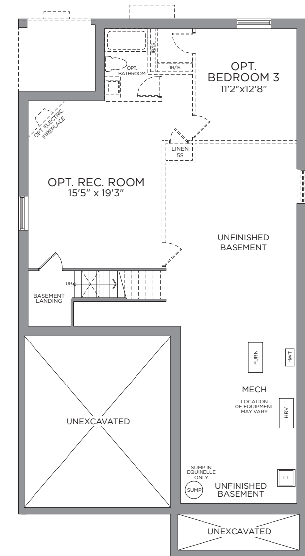
STANDARD BASEMENT ELEV. B OPT. FINISHED BASEMENT FINISHED AREA 718 SQ. FT.
