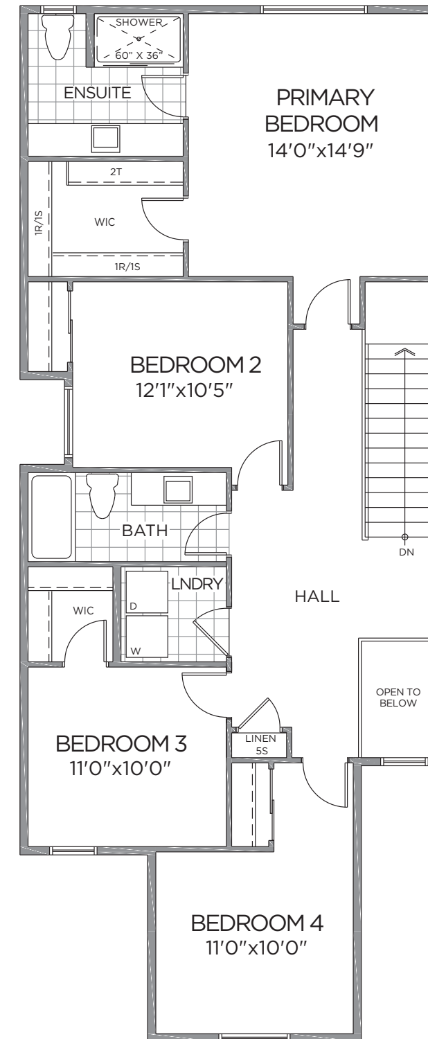
SECOND FLOOR ELEV. B
