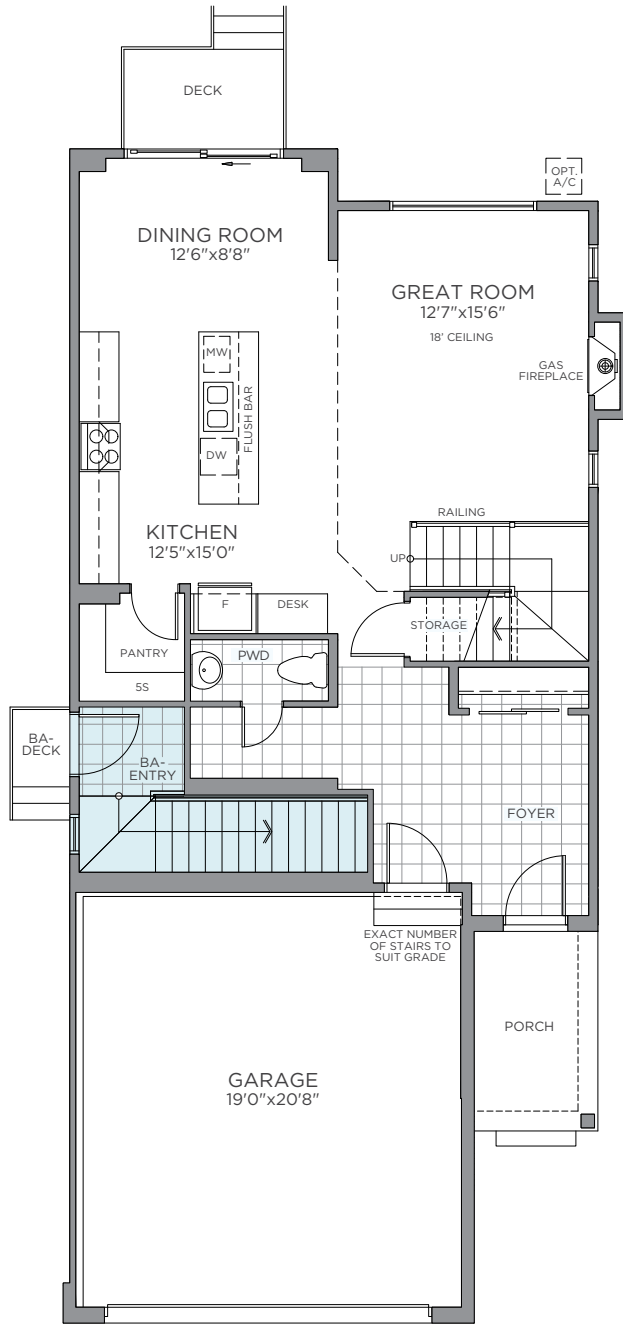
GROUND FLOOR
